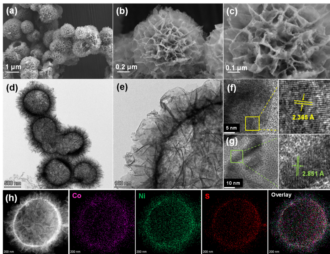
Fig. 2 (a–c) SEM and (d–g) TEM images of (Co 1 Ni 2 )S 4 and (h) elemental mapping of Co, Ni, and S elements of (Co 1 Ni 2 )S 4 .
