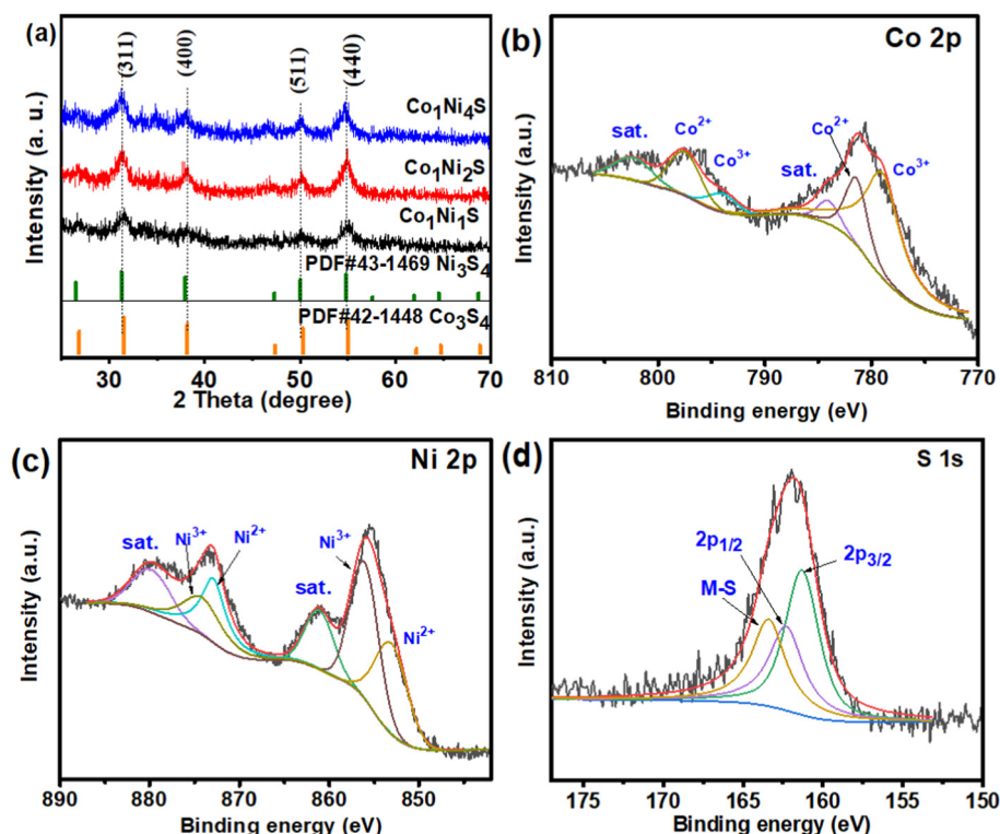
Fig. 3 (a) XRD for \text{Co}_x\text{Ni}_{3-x}\text{S}_4 and XPS spectra of (b) the Co 2p, (c) Ni 2p, and (d) S 1s for (\text{Co}_1\text{Ni}_2)_2\text{S}_4 .
