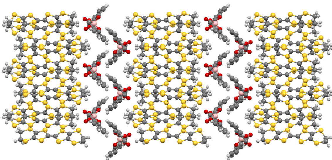
Fig. 10 Double anion layer in \kappa\text{-(BEDT-TTF)}_2[B_6RS(\text{salicylate})_2] .
