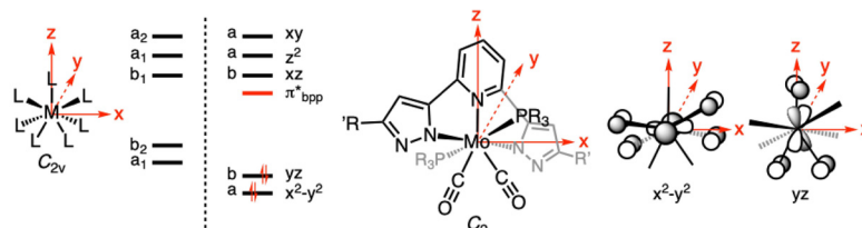
Fig. 4 d orbital splitting for a model C_{2v} ML_7 complex (left) and qualitative prediction of the frontier orbitals for the series of complexes 4a–c and 5a–c with depiction of possible overlap of filled d orbitals with ligands' \pi -shaped MOs.
