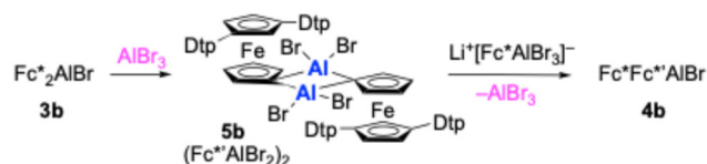
Scheme 3 Reaction of 3b with AlBr 3 to yield dibromoaluminum dimer 5b , which could subsequently be converted to 4b .
