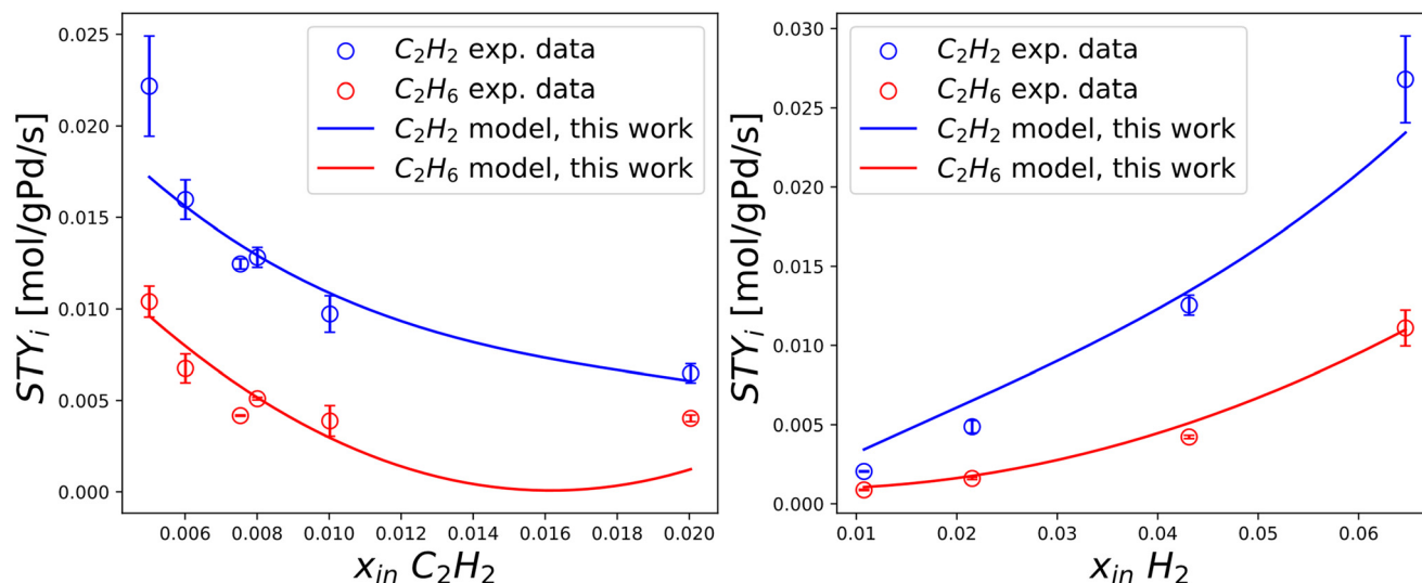
Fig. 8 Experimentally measured and modelled space-time yields of C_2H_2 and C_2H_6 (STY C_2H_2 [mol g Pd -1 s -1 ] and STY C_2H_6 [mol g Pd -1 s -1 ]) plotted against single manipulated operating variables. Includes experimental data by Urmes et al. and model simulation results by this work. Left) Trends vs. inlet molar fraction of C_2H_2 obtained at 323 K, i.e. 50 °C. Right) Trends vs. inlet molar fraction of H_2 obtained at 323 K, i.e. 50 °C. The standard deviation of experimental measurements is reported through error bars for points whose reproducibility has been verified through at least two repeated experiments.
