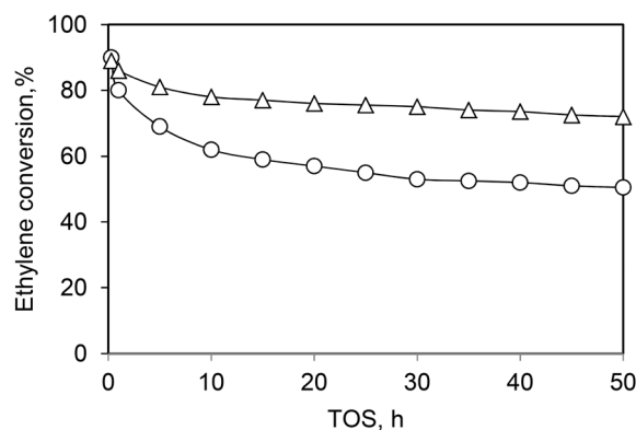
Fig. 10 Ethylene conversion vs. time on stream in the presence of (○) C 2 H 4 + N 2 and (△) C 2 H 4 + N 2 + H 2 over the Ni-ASA catalyst. Reaction conditions: T = 250 °C, P = 1.5 MPa, WHSV = 1.1 h -1 . This scheme has been reproduced from ref. 39.
