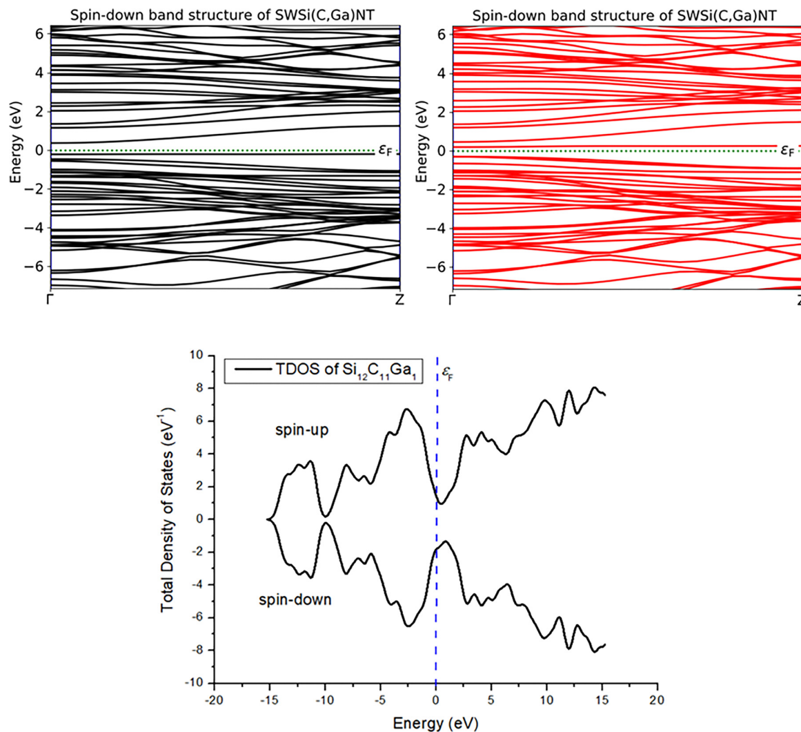
Fig. 9 The calculated spin-up (black) and spin-down (red) band structures, and TDOS diagram for \text{Si}_{12-x}\text{Ga}_x NTs.
