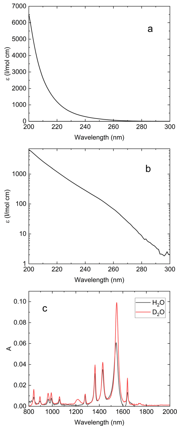
Fig. 1 Ultraviolet and infrared absorption spectra of aqueous acrylate. (a) UV absorption spectrum of aqueous acrylate recorded against an H 2 O reference shown on a linear absorption scale. (b) UV absorption spectrum of acrylate dissolved in H 2 O recorded against H 2 O shown on a logarithmic absorption scale. The absorption scales in (a) and (b) have been calibrated to the extinction coefficients reported in ref. 23. (c) IR steady state absorption spectra of acrylate dissolved in H 2 O and D 2 O recorded against H 2 O and D 2 O references.
