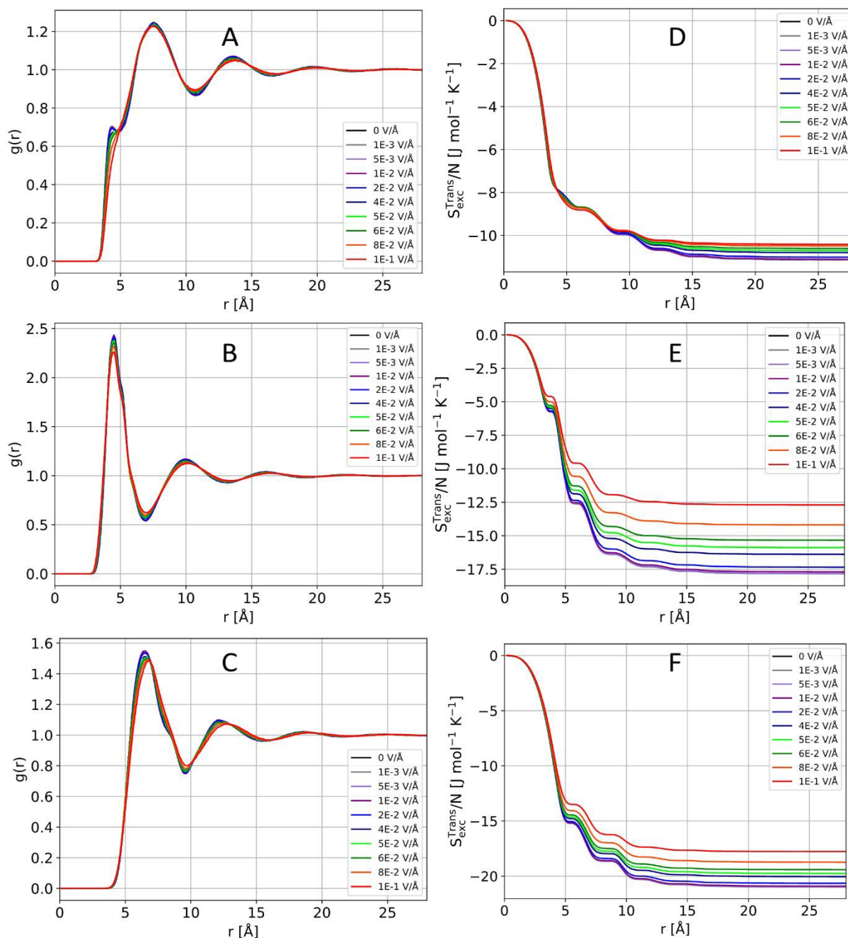
Figure 4. Radial distribution functions between [C_2C_{1im}]-[C_2C_{1im}] , [C_2C_{1im}]-[Cl] and [Cl]-[Cl] on panels A, B and C, respectively, as a function of EEF at 380K. Estimates of translation excess entropy in J/mol\cdot K as a function of radius from [C_2C_{1im}]-[C_2C_{1im}] , [C_2C_{1im}]-[Cl] , and [Cl]-[Cl] structure on panels D, E and F, respectively, for multiple EEFs at 380K computed with Eq. [11].
