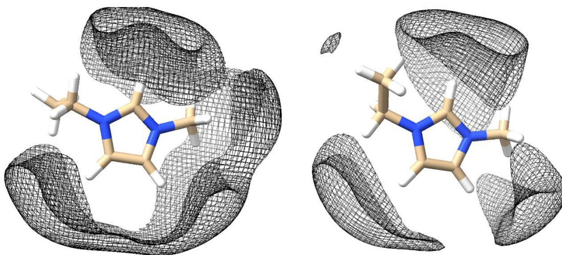
Figure 2. Spatial distribution function of the [Cl] anion around the center of mass of the [C 2 C 1 im] cation showing an iso-surface with a cutoff 3 times the bulk density. The left panel shows the spatial distribution function without an EEF. The right panel shows the spatial distribution when an EEF of 1 \times 10^{-1} V/Å is present.
