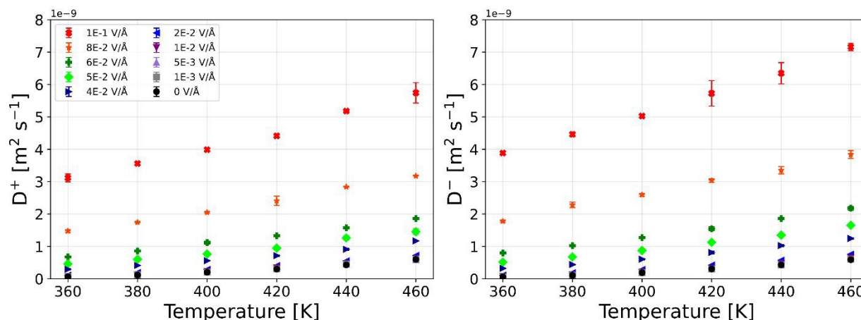
Figure 3. Self-diffusion coefficients for [C_2C_1im] and [Cl] on the left and right panel respectively for multiple temperatures across different EEFs. At high EEF there is a substantial increase of the self-diffusion coefficient for both ions. Both panels share the same legend. For both ions, self-diffusion coefficients are unaffected and overlap for EEF up to 2 \times 10^{-2} V/Å. Only until an EEF of 4 \times 10^{-2} V/Å or larger is applied that changes in self-diffusion coefficients are observed. Error bars represent the standard deviation between three independent replicates of [C_2C_1im][Cl] .
