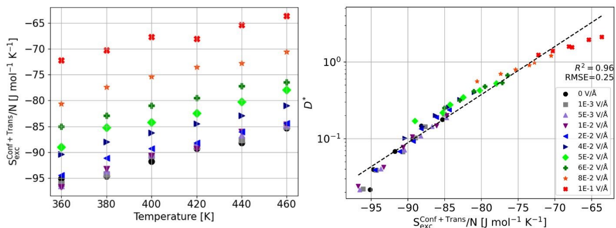
Figure 7. Excess entropy scaling test for IL self-diffusion coefficients across temperatures and EEF for replicate 3 as a representative example. Left) Partial molar configurational and translational excess entropy in [\text{J/mol}\cdot\text{K}] of the IL versus temperature across EEF. As the temperature and the EEF increase, the magnitude of excess entropy decreases. Right) Reduced combined self-diffusion coefficient versus partial molar excess entropy. As EEF increases, the magnitude of partial molar excess entropy is less negative which indicates an increase in dynamics. The computed excess entropy and self-diffusion coefficients across EEF and temperatures follow a Dzugutov scaling relationship (black fitted dashed line) with c_1 = 3.9 \times 10^4 and c_2 = 1.4 \times 10^{-1} [\text{J/mol}\cdot\text{K}]^{-1} obtained from the fit to the equation in the right panel. The dashed black line is the obtained fit of the equation in the right panel.
