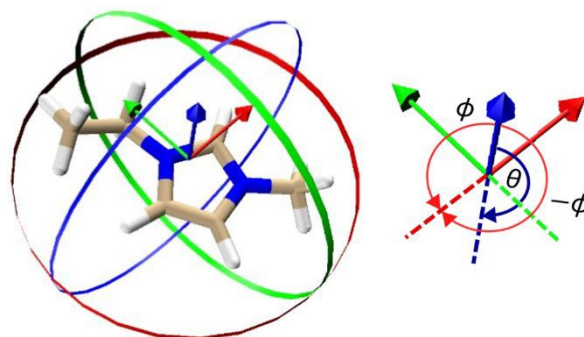
Figure 1. Left) cation reference axis is depicted with red, green, and blue arrows representing the positive x , y , and z axes. Colored rings of radius 4.5 Å serve as visual aids: the red ring indicates variations in \phi , and the blue and green rings illustrate variations in \theta . Right) spherical reference axis showing how \theta and \phi vary. Intersections of the colored rings correspond to specific \theta and \phi values—for example, where green and blue rings meet in the positive z -direction \theta=0 and where red and blue rings meet in the positive x -direction \theta=\pi/2 and \phi=0 . The point where green and red rings meet in the positive y -direction corresponds to \theta=\pi/2 and \phi=\pi/2 while the point where the rings meet again in the negative y direction correspond to \theta=\pi/2 and \phi=-\pi/2 .
