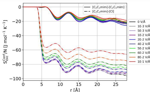
Figure 6. Estimate of configurational excess entropy in \text{J/mol}\cdot\text{K} as a function of radius from [\text{C}_2\text{C}_1\text{im}]\text{-}[\text{Cl}] and [\text{C}_2\text{C}_1\text{im}]\text{-}[\text{C}_2\text{C}_1\text{im}] structure at 380 K across EEFs for replicate 1 as a representative example. The solid and dot dashed lines represent the configurational excess entropy between [\text{C}_2\text{C}_1\text{im}]\text{-}[\text{C}_2\text{C}_1\text{im}] and [\text{C}_2\text{C}_1\text{im}]\text{-}[\text{Cl}] computed from g_{\text{conf}}(r|\omega_1) respectively with Eq. [13]. The configurational excess entropy contribution from the [\text{C}_2\text{C}_1\text{im}]\text{-}[\text{C}_2\text{C}_1\text{im}] configurational correlations is smaller and less sensitive to the EEF compared to the configurational excess entropy from the [\text{C}_2\text{C}_1\text{im}]\text{-}[\text{Cl}] configurational correlations.
