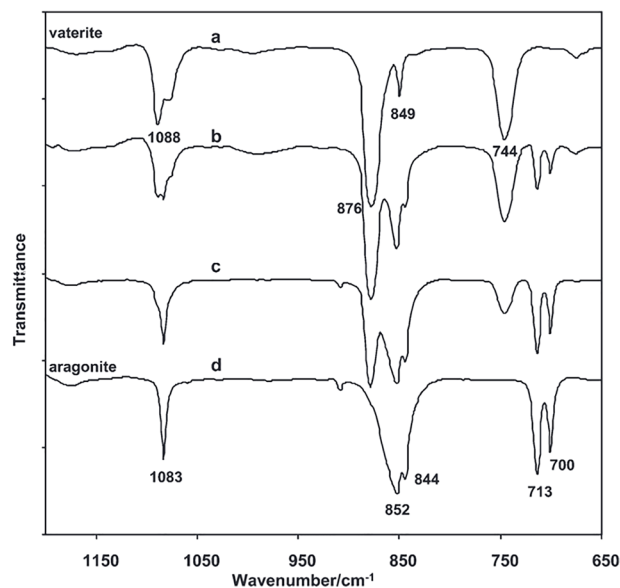
Fig. 8 FTIR spectra (650–1200 \text{cm}^{-1} ) of (a) the vaterite sample, and when it was refluxed in distilled water for (b) 30 min, (c) 60 min, and (d) 75 min. Adapted from ref. 27 with permission from American Chemical Society, copyright 2010.
