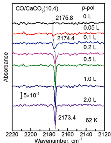
Fig. 11 IRRAS spectra with p -polarized light for CO adsorbed on the calcite (10.4) surface at 62 K with increasing exposures (0–2 L). Adapted from ref. 34 with permission from Royal Society of Chemistry, copyright 2021.
