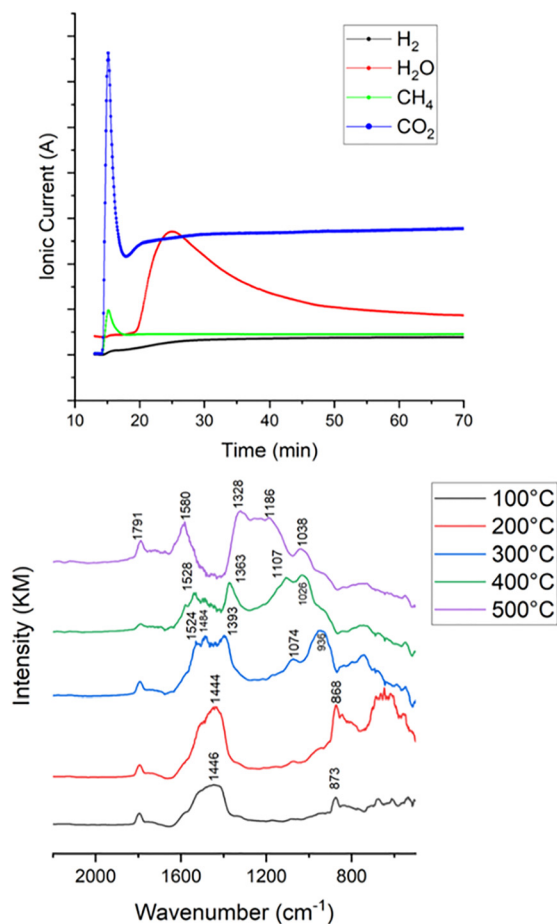
Fig. 12 Operando \text{CO}_2 methanation at 400 °C on Ni/dolomite: (Top) evolution of mass spectroscopy signal with reaction time. (Bottom) In situ DRIFT spectra as a function of catalyst temperature. Adapted from ref. 37 with permission from Elsevier B. V., copyright 2024.
