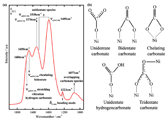
Fig. 13 (a) Infrared spectra of \text{CO}_2 adsorbed on the Ni-hydrotalcite derived catalyst and (b) possible species appeared in the \text{CO}_2 adsorption experiment. Adapted from ref. 38 with permission from Elsevier B. V., copyright 2023.
