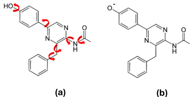
Fig. 1 (a) Coelenteramide's protonated species, 2H . Here, the most flexible internal coordinates are indicated in red; (b) coelenteramide's anionic species, 20 - .
