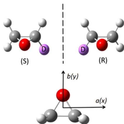
Fig. 1 \text{C}_2\text{H}_3\text{DO} (monodeutero-oxirane): structure and axes. In the lower part the c(z) axis is perpendicular to the plane pointing towards the observer in a right-handed coordinate system. The D atom is hidden behind the plane (here, the axes are shown for the symmetrical \text{C}_2\text{H}_4\text{O} , in \text{C}_2\text{H}_3\text{DO} they are moved away from the symmetrical position).
