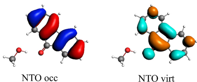
Fig. 6 Calculated NTO of B3LYP/TZ2P/TDA-level for fluorenone–methanol, where the occupied (left) and virtual NTO (right) represent 98% of the density-change for the excitation.
