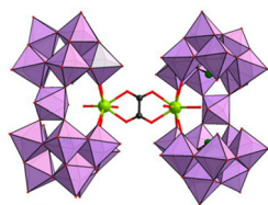
Fig. 10 Polyhedral/ball-and-stick representation of \text{K}_{17}\text{Na}_2\text{H}_5[(\text{As}_2\text{W}_{19}\text{O}_{67}(\text{H}_2\text{O}))\text{Ln}(\text{H}_2\text{O})_2]_2(\text{C}_2\text{O}_4)] \cdot 87\text{H}_2\text{O} .
