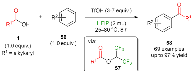
Scheme 9 HFIP esters as reactive intermediates.
