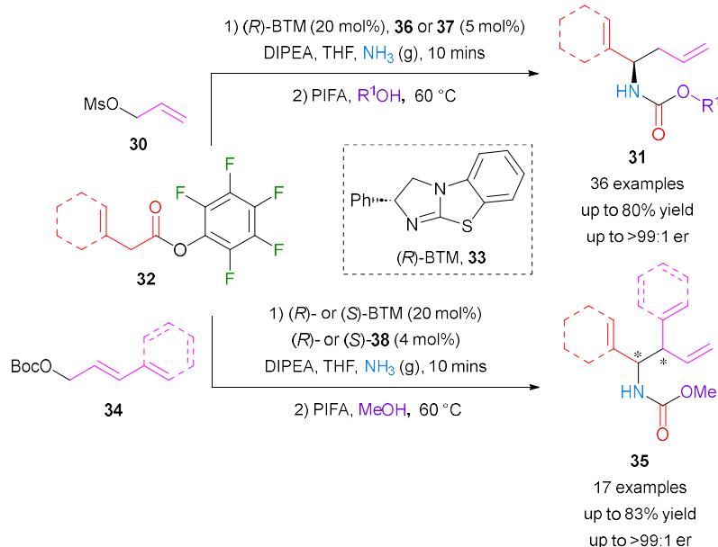
Scheme 7 The synthesis of linear and branched N -substituted homoallylic amines from PFPh esters.
