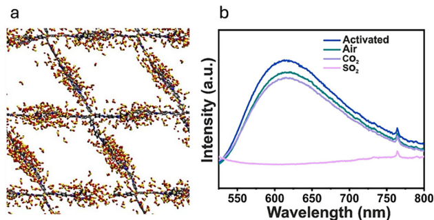
Fig. 4 SomoCOF-9: (a) structural interaction with SO 2 molecules, (b) photoluminescence emission spectrum with air, CO 2 , and after SO 2 . 10
