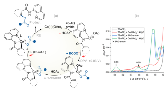
Scheme 3 Plausible mechanism of cobalt electro-catalyzed C–H acyloxylation. (a) Proposed catalytic cycle. (b) Differential pulse voltammetry of reaction mixture components under model conditions.
