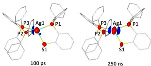
Fig. 2. Photodifference ( F^{\text{ON}} - F^{\text{OFF}} ) maps derived from the Laue experiment indicating electron-density changes 100 ps and 250 ns after excitation plotted on the AgPPPS ground-state geometry. Isosurfaces represent regions with electron density difference of at least \pm 0.35 \text{ e-}\text{\AA}^{-3} (left) or \pm 0.55 \text{ e-}\text{\AA}^{-3} (right) (blue – positive, red – negative).
