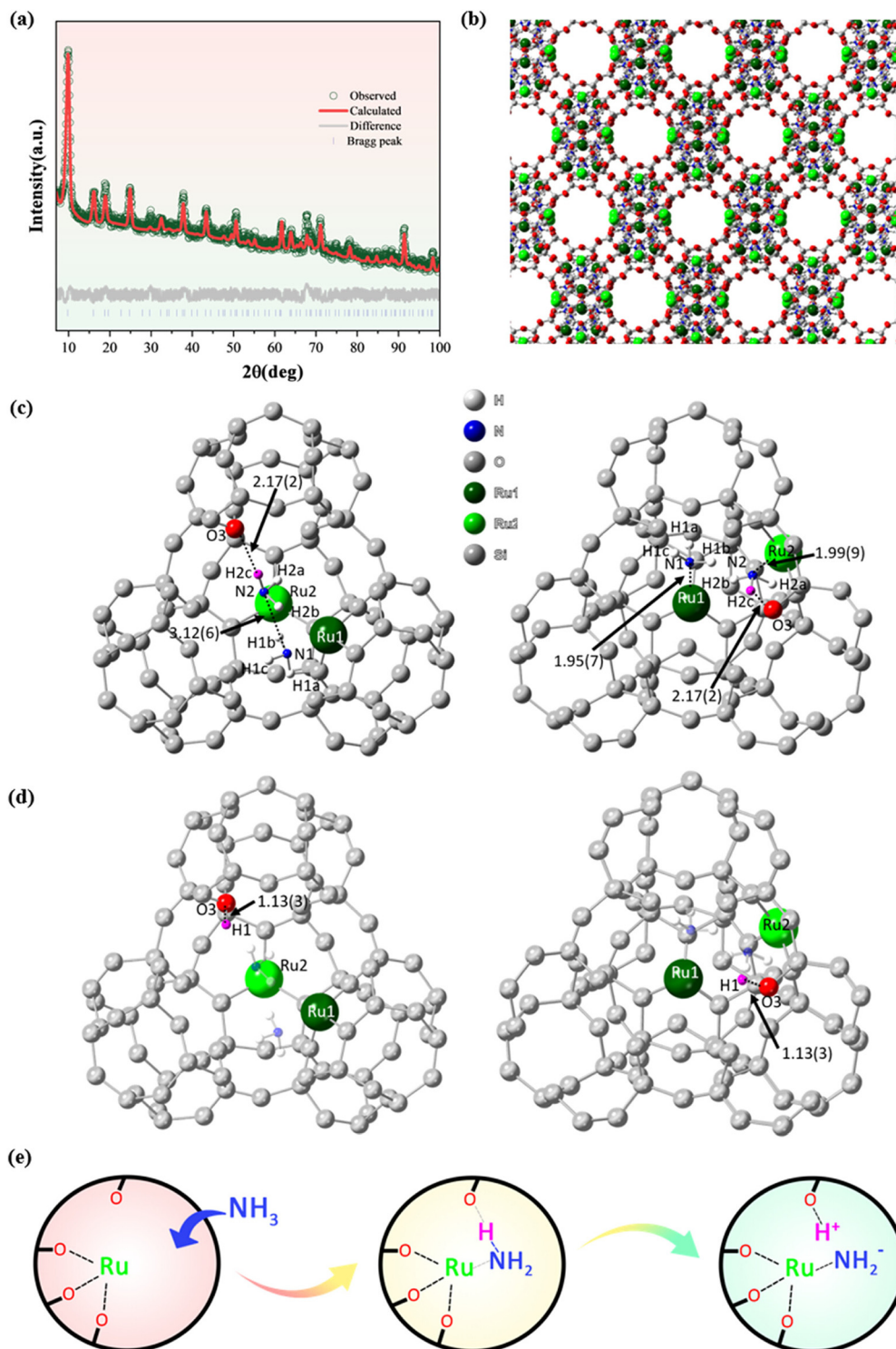
Fig. 15 (a) Original and Rietveld refinement fit of NPD data of X1.4H-RT ( R_{\text{wp}} = 2.375\% , R_{\text{exp}} = 1.865\% , \text{gof} = 1.2736 ). (b) Zeolite structure showing the determined proton sites and \text{NH}_3 molecules of X1.4H-RT via NPD-Rietveld refinement. The atoms are labeled according to the element (dark green = Ru1, light green = Ru2, red = O, gray = Si and Al, blue = N and white = H). (c) Zeolite structure with the determined \text{NH}_3 molecules of X1.4H-RT with the bond length information (in Å) via NPD-Rietveld refinement. All O atoms are turned into gray color except the O atom (O3) that is located close to the proton H2c (in pink) of the adsorbed \text{NH}_3 of Ru2 and is able to undergo the FLP-type dissociation mechanism. (d) Zeolite structure containing regenerated proton sites on O atoms and \text{NH}_3 molecules of X1.4H-450 with given bond length information (in Å) via NPD-Rietveld refinement. All O atoms are turned into gray color except the O atom (O3) that undergoes the FLP-type dissociation mechanism and the corresponding proton H1 (in pink). (e) Proposed FLP-type mechanism for the N-H cleavage that occurred between \text{NH}_3 gas and the Ru sites in the Ru-loaded 13X zeolite. (Reproduced from ref. 107. Copyright (2023), with permission from ACS Publications).
