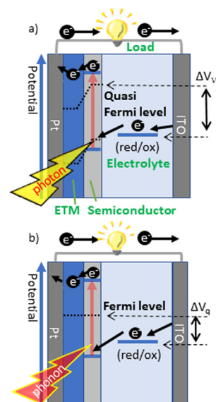
Fig. 5 Schematic image of the output potential by (a) photoexcitation and (b) thermal excitation. ETM: electron transport material 43 (Copyright © 2020 The Chemical Society of Japan).
