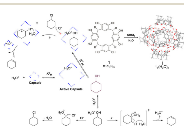
Fig. 3 Catalysis of the dehydration of cyclohexanol to produce cyclohexene using the capsule I. Adapted from ref. 59 with permission, copyright 2020, American Chemical Society.
