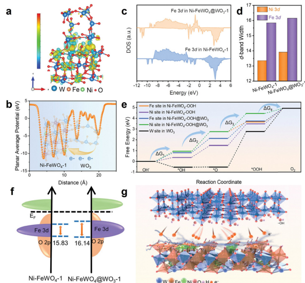
Fig. 5 (a) Charge density difference of \text{Ni-FeWO}_4@\text{WO}_3 -1. (b) Plane-average electron difference diagram of the interface between \text{Ni-FeWO}_4 and \text{WO}_3 -1. (c) Projected DOS of Fe 3d in \text{Ni-FeWO}_4 -1 and \text{Ni-FeWO}_4@\text{WO}_3 -1. (d) The d-band widths of Fe 3d and Ni 3d in \text{Ni-FeWO}_4 -1 and \text{Ni-FeWO}_4@\text{WO}_3 -1. (e) Free energy profiles of different OER intermediates at 0 V for the Fe site. (f) Variation of the d-band widths of Fe 3d. (g) Schematic illustration of the electron barrier layer for the protection of Fe and Ni sites in \text{Ni-FeWO}_4@\text{WO}_3 . Reproduced with permission of ref. 71 copyright 2023, Wiley-VCH.
