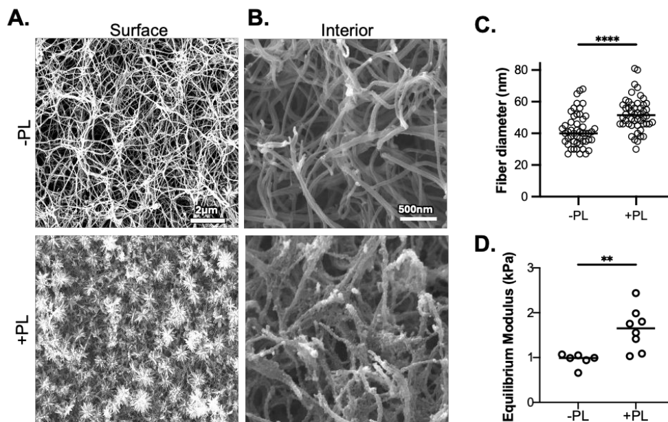
Figure 2. Scanning electron micrographs of fibrin gels without or with platelet lysate (PL) obtained [A] on the surface or [B] within gels. Scale bar = 2 μm and 500 nm, respectively. [C] Quantification of fibrin fiber diameter within the interior of the gel. n > 40 fibers per group from 3 images. [D] Equilibrium modulus of fibrin gels without or with PL augmentation. n = 6-8 per group. ** p < 0.01 , **** p < 0.0001 .
