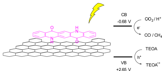
Fig. 7 Reduction of CO 2 over QA/rGO photocatalyst, and schematic representation of CO 2 reduction to CO and CH 4 , coupled with oxidation of triethanolamine (TEOA); the potential of the conduction and valence bands (CB and VB, respectively) are reported versus the reversible hydrogen electrode. 49
