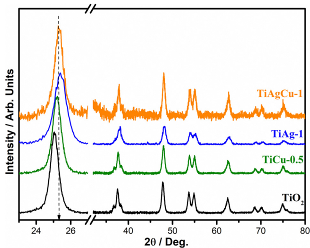
Fig. 1 Wide angle XRD patterns of mesoporous \text{TiO}_2 , \text{Ag}/\text{TiO}_2 (TiAg-1), \text{Cu}/\text{TiO}_2 (TiCu-0.5) and TiAgCu-1 nanocomposites. A significant shift and broadening of the (101) diffraction feature is observed with TiAg-1 and TiAgCu-1. All the diffraction features are attributed to the anatase phase of \text{TiO}_2 .
