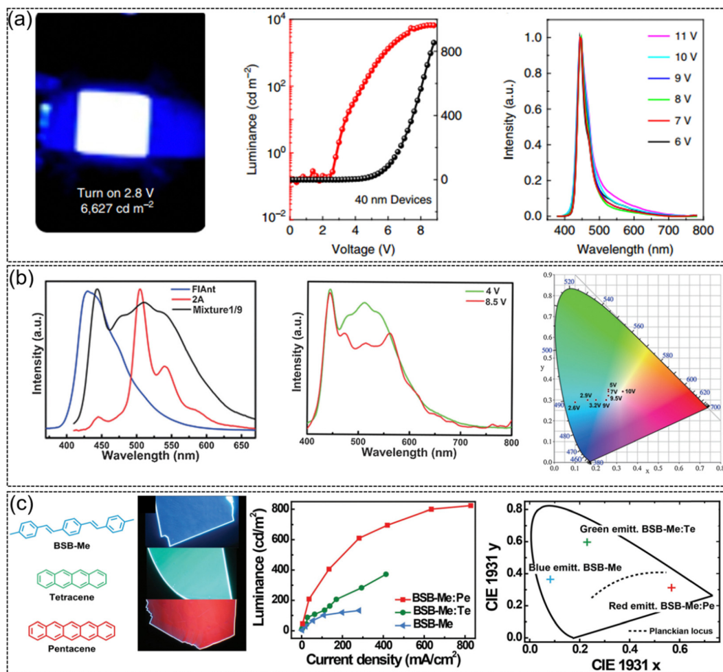
Fig. 9 Representative applications in OLEDs. (a) Strong blue emission from OLEDs based on DPA (2 mm \times 2 mm), current density–voltage–luminance characteristics of the OLEDs and EL spectra operated at different voltages. Reproduced with permission. 39 Copyright 2015, Springer Nature. (b) EL spectra in OLEDs based on FlAnt, 2A, and mixture1/9, EL spectra of mixture1/9 at 4 and 8.5 V and CIE coordinates at different driving voltages in OLED devices based on mixture1/9. Reproduced with permission. 66 Copyright 2016, John Wiley and Sons. (c) Chemical structures and top-view photographs of BSB-Me, BSB-Me:Te, and BSB-Me:Pe organic crystals under UV-light irradiation, EL performance of BSB-Me, BSB-Me:Te, and BSB-Me:Pe single-crystal-based OLEDs and corresponding 1931 CIE coordinate diagrams of blue, green, and red light emission with CIE coordinates of (0.56, 0.31), (0.23, 0.59), and (0.08, 0.36), respectively. Reproduced with permission. 137 Copyright 2017, John Wiley and Sons.
