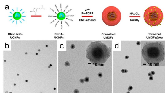
Fig. 13 (a) Illustration depicting the formation of core–shell UMOF@Au NPs. TEM images of (b) carboxylic acid stabilized UCNPs in aqueous solution, UMOF NPs (c), and UMOF@Au NPs (d). (Panels a–d) Reproduced with permission. 6 Copyright 2020, American Chemical Society.
