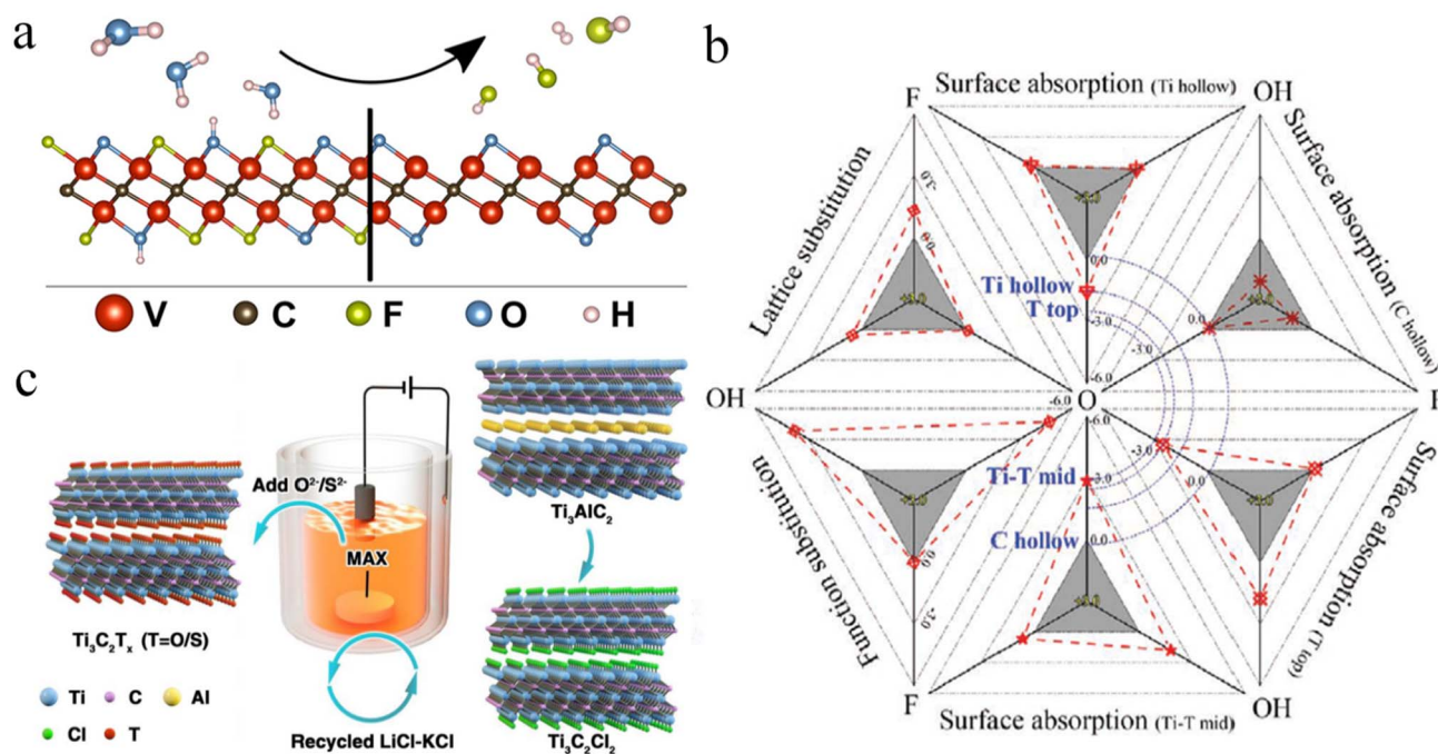
Fig. 8 (a) Removal of fluoride terminations by gas hydrolyzation, reproduced from ref. 147 with permission from American Chemical Society, copyright 2022. (b) Simulation with nitrogen dopants in \text{Ti}_3\text{C}_2 , reproduced from ref. 149 with permission from Wiley, copyright 2020. (c) MXene synthesis by molten salt etching, reproduced from ref. 151 with permission from Wiley, copyright 2021.
