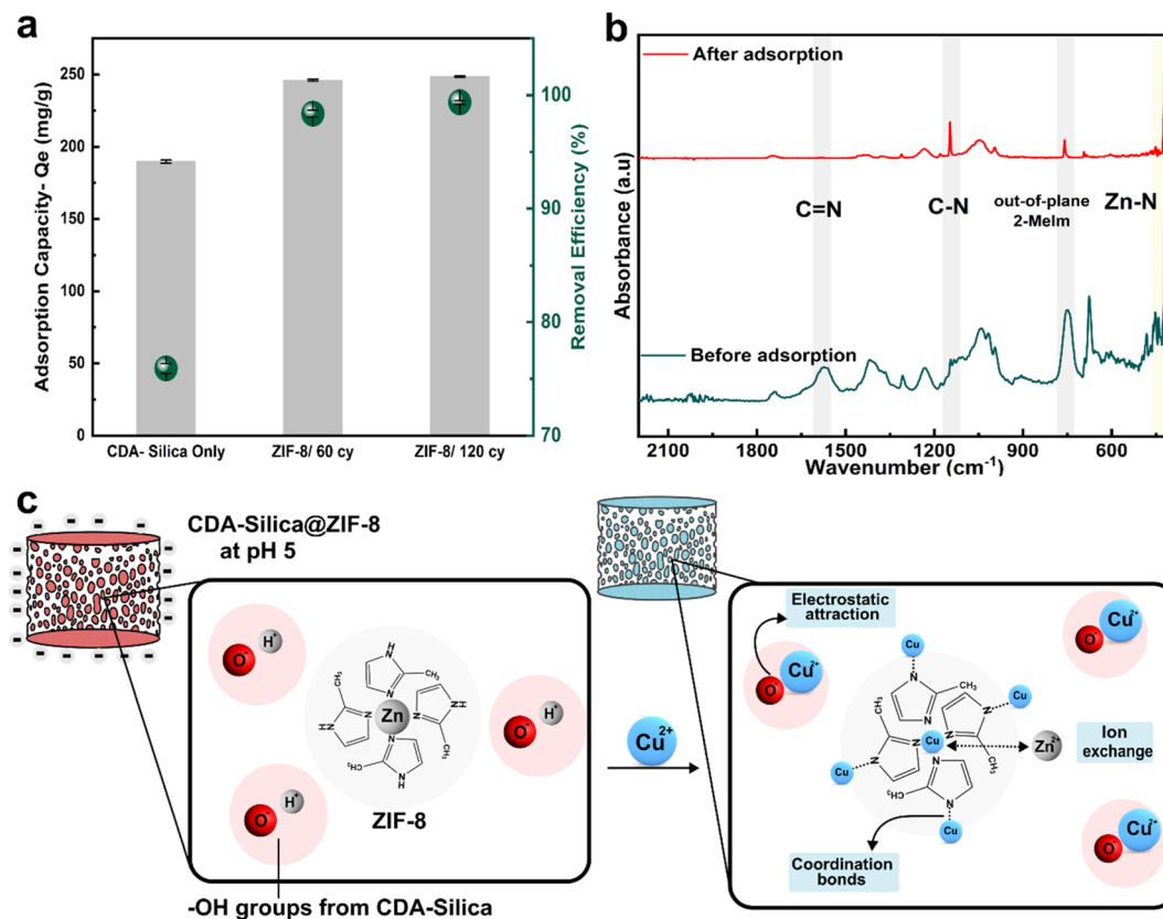
Fig. 5 Heavy metal removal: (a) adsorption capacity (mg g -1 ) and removal efficiency (green circles, %) for 20 mg of the adsorbent (aerogel) load in 100 mg L -1 of stock solution of Cu 2+ ions and (b) FTIR spectra of CDA-silica@ZIF-8/120cy before and after adsorption of Cu 2+ . Note that all three samples in (a) are aerogels. (c) Adsorption mechanism depicting ion-exchange with Zn, formation of coordination complex of Cu with N atoms of ZIF-8, and electrostatic interactions between hydroxyl groups of CDA-silica and Cu.
