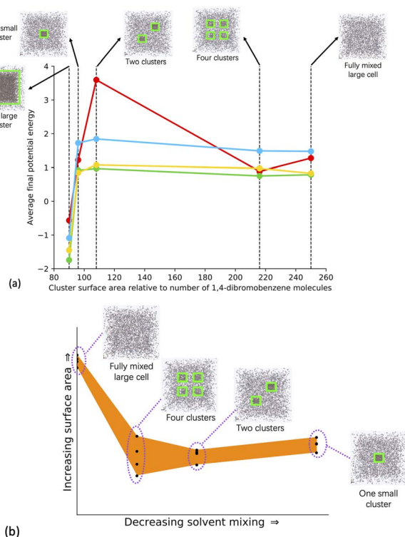
Fig. 4 (a) Average final potential energy relative to the number of DBB molecules for models generated in different solvents. Key: toluene – blue, THF – yellow, 1,4-dioxane – green, DMF – red. (b) Plot of the surface area against the solvent mixing for all the models generated for the phase separated systems. The different structural configurations modelled in the phase separated systems are shown as insets. The yellow boxes around each cluster are present for clarity. In each model the number of respective solvent molecules and cell size is the same. The one large cluster Solvent/monomer phase interface system has 15× more monomer and catalyst units than the phase separated system models. See Table SI.10† for full details.
