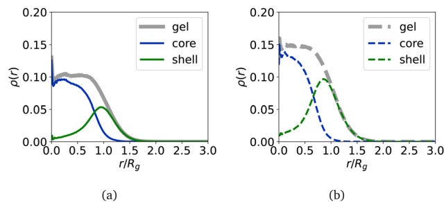
Fig. 10 Density profiles for magnetic core-shell MNGs with MNPs both in the core and in the shell, \lambda = 6 , K_{\text{sh}} = 100 . (a) M_{\text{sh}} = 10 ; (b) M_{\text{sh}} = 20 . The grey colour corresponds to all particles in the nanogel, the blue colour is chosen for particles in a core, and the green colour is used for particles in a shell.
