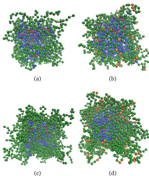
Fig. 9 Snapshots for different models of core-shell magnetic nanogels: (a) magnetic core with shell polymer length M_{\text{sh}} = 10 , (b) magnetic core and shell with shell polymer length M_{\text{sh}} = 10 , (c) magnetic core with shell polymer length M_{\text{sh}} = 20 , (d) magnetic core and shell with shell polymer length M_{\text{sh}} = 20 . Blue particles – nonmagnetic particles of a core, green particles – nonmagnetic particles of a shell, red particles – magnetic particles of a core, orange particles – magnetic particles of a shell.
