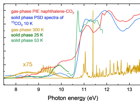
Fig. 5 Comparison of the PIE curve of naphthalene- \text{CO}_2 with solid phase photon-stimulated desorption (PSD) spectrum of ^{13}\text{CO}_2 , 20 \text{CO}_2 gas-phase spectrum 39 and \text{CO}_2 solid phase absorption spectra. 40–42
