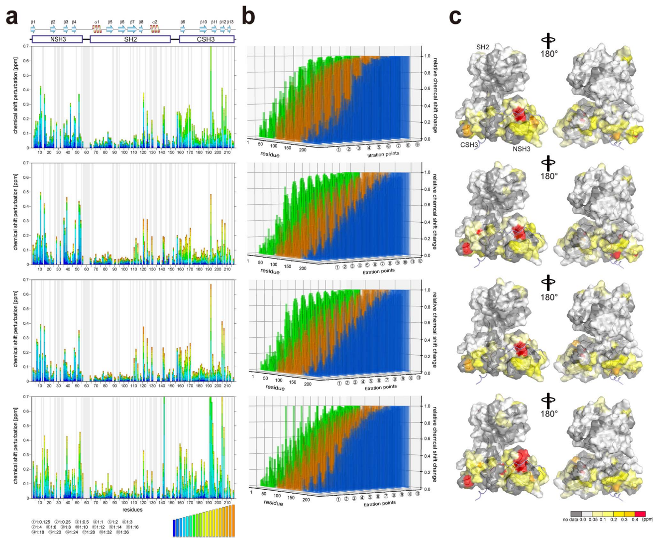
Fig. 2 Plots of chemical shift perturbation of backbone ^1\text{H} and ^{15}\text{N} nuclei of GRB2 upon the titration with S4, S5, S9, and S10 PRMs. (a) Bar plots of chemical shift perturbation of backbone ^1\text{H} and ^{15}\text{N} nuclei of GRB2 upon the titration with S4, S5, S9, and S10 PRMs. The mean shift difference \Delta\delta_{\text{ave}} was calculated as [(\Delta\delta^1\text{H})^2 + (\Delta\delta^{15}\text{N}/5)^2]^{1/2} where \Delta\delta^1\text{H} and \Delta\delta^{15}\text{N} are the chemical shift differences (ppm) between GRB2 on its own and in the presence of the PRMs. The bar graphs are colour-coded according to the protein-peptide concentration ratio and are overlaid. The proline residues as well as the residues for which ^1\text{H} - ^{15}\text{N} correlation cross-peaks were not analysed due to signal overlap or other reasons are shown in grey. The secondary structures of GRB2 are also shown. (b) Chemical shift perturbation 3D bar plots with an added axis for titration points to the plots of figure (a). The vertical, horizontal, and height axes represent the residue number, titration point, and chemical shift perturbation, respectively. NSH3, SH2, CSH3, and the linker regions are shown in green, orange, blue, and grey, respectively. (c) Chemical shift perturbation upon the titration with S4, S5, S9, and S10 PRMs represented on the crystal structure of GRB2 (PDB ID: 1GRI).
