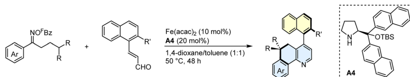
(a) Construction of axially chiral pyridine-based biaryls
