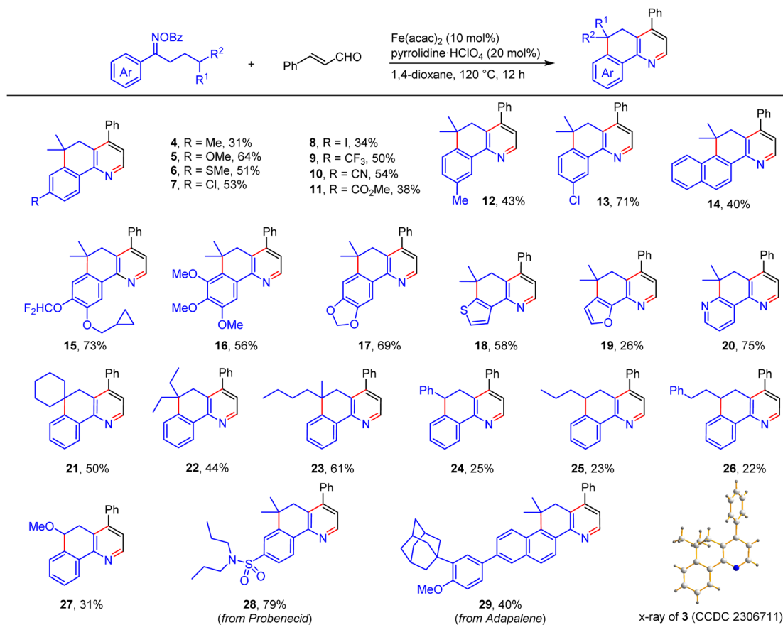
Scheme 3 Substrate scope of the oxime esters. Reaction conditions: oxime ester (0.6 mmol), enal (0.2 mmol), Fe(acac) 2 (10 mol%), pyrrolidine·HClO 4 (20 mol%), 1,4-dioxane (2 mL), 120 °C, 12 h, under N 2 .
