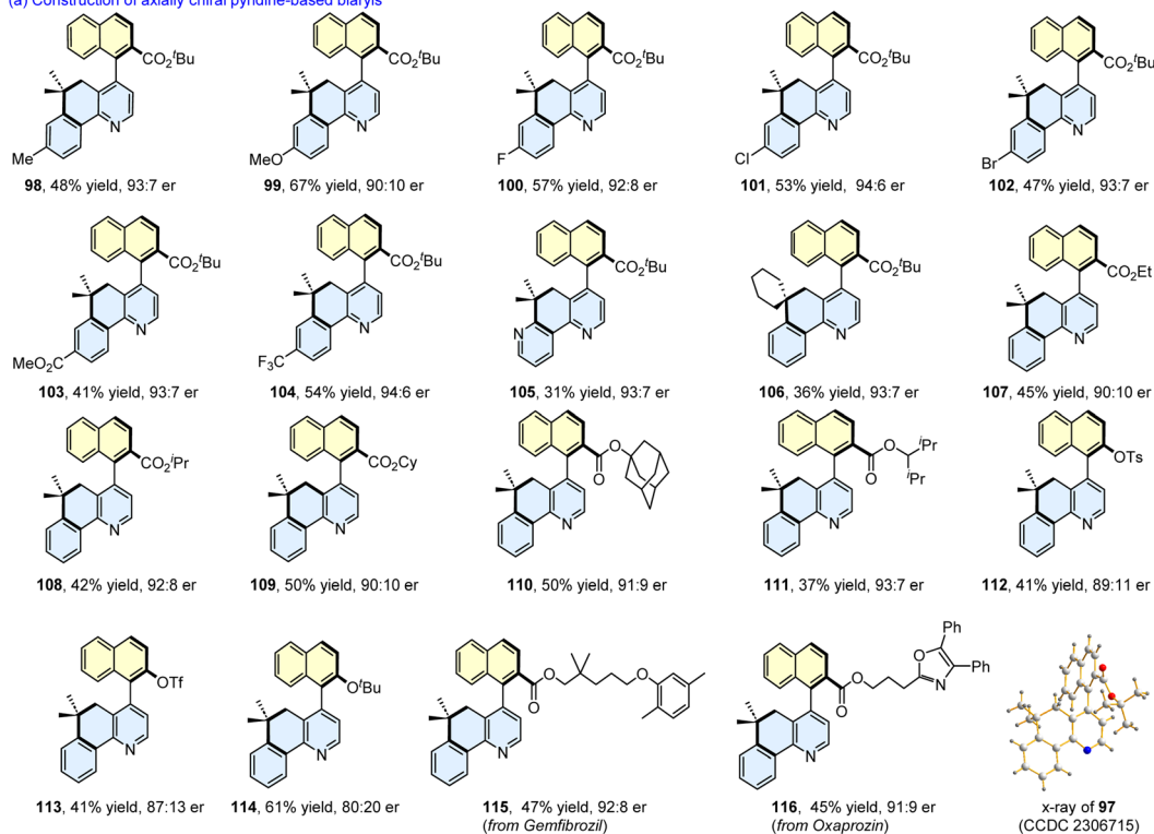
(b) Synthetic transformations of axially chiral pyridine-based biaryls
