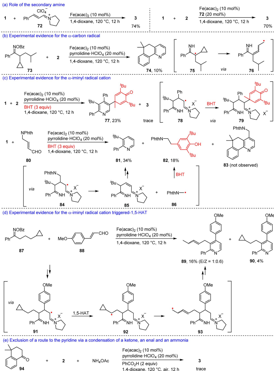
Scheme 6 Mechanistic studies ( X = \text{ClO}_4 , OBz, or acac).
