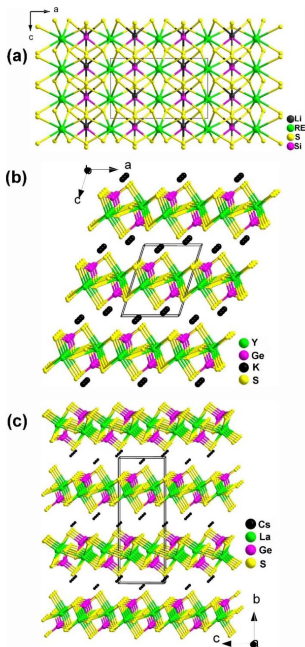
Fig. 11 Structures of (a) \text{LiRESiS}_4 (space group: \text{Ama}2 ), (b) \text{KYGeS}_4 (space group: \text{P}2_1 ), and (c) \text{CsLaGeS}_4 (space group: \text{P}2_12_12_1 ) with the unit cell outlined.
