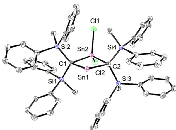
Fig. 6 Molecular structure of 5\text{Cl} in the crystalline state with thermal ellipsoids at 50% probability; hydrogen atoms are omitted for clarity. Selected bond lengths [ \text{\AA} ] and angles [ ^\circ ] for 5\text{Cl} : \text{Sn}1 \cdots \text{Sn}2 : 3.1022(5) , \text{C}1\text{--}\text{Sn}1 : 2.313(2) , \text{C}2\text{--}\text{Sn}1 : 2.301(2) , \text{C}1\text{--}\text{Sn}2 : 2.163(2) , \text{C}2\text{--}\text{Sn}2 : 2.173(2) , \text{C}1\text{--}\text{Si}1 : 1.905(2) , \text{C}1\text{--}\text{Si}2 : 1.888(2) , \text{C}2\text{--}\text{Si}3 : 1.902(2) , \text{C}2\text{--}\text{Si}4 : 1.909(2) , \text{C}1\text{--}\text{Sn}1\text{--}\text{C}2 : 87.93(8) , \text{C}1\text{--}\text{Sn}2\text{--}\text{C}2 : 95.22(8) , \text{Sn}1\text{--}\text{C}1\text{--}\text{Sn}2 : 87.67(8) , and \text{Sn}1\text{--}\text{C}2\text{--}\text{Sn}2 : 78.76(8) .
