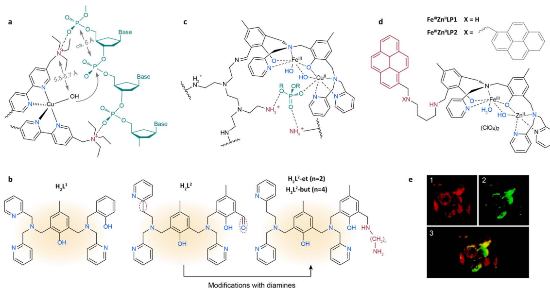
Fig. 5 (a) The proposed intermediate of DNA cleavage by [Cu(L1)_2(Br)](ClO_4)_5 \cdot 6H_2O , where L1 is 5,5'-di((triethylammonio)methyl)-2,2'-dipyridyl. 109 Adapted with permission from ref. 109. Copyright 2006 The Royal Society of Chemistry. (b) The structures of H_2L^1 , H_2L^2 , H_2L^2 -et and H_2L^2 -but. 112 Adapted with permission from ref. 112. Copyright 2017 The Royal Society of Chemistry. (c) The proposed structure for the FeCuI-PEI system with a bound phosphate diester. 111 Adapted with permission from ref. 111. Copyright 2013 American Chemical Society. (d) The structures of Fe^{III}Zn^{II}LP1 and Fe^{III}Zn^{II}LP2 . 113 (e) Accumulation of Fe^{III}Zn^{II}LP1 in lysosomes, where Fe^{III}Zn^{II}LP1 is pseudocolored in green (1) and the lysotracker in red (2). 113 Adapted with permission from ref. 113. Copyright 2017 American Chemical Society. The substrate and first and second coordination spheres are colored in green, blue and red, respectively, unless specified.
