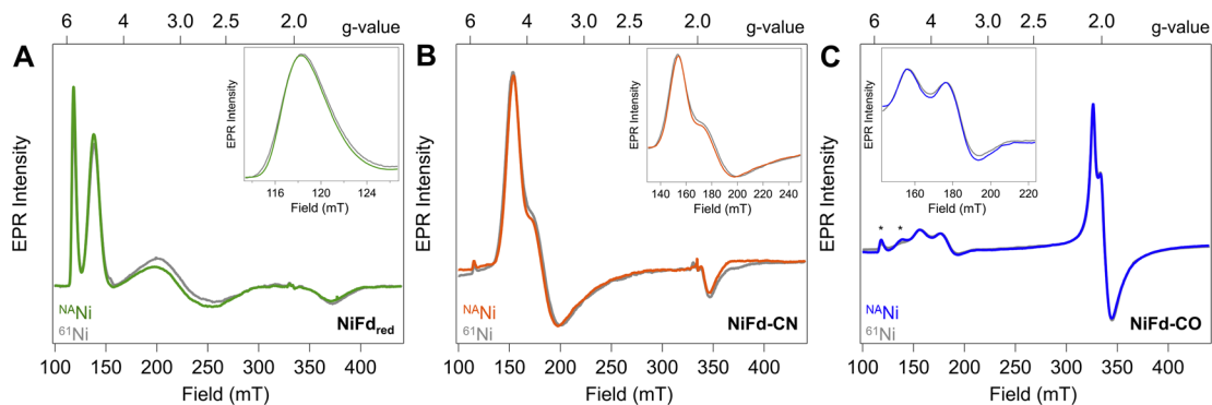
Fig. 2 CW X-band EPR spectra ( \nu = 9.37 GHz, P_{\text{MW}} = 20 mW, T = 8.0 K) of natural abundance (colored traces) and ^{61}\text{Ni} -isotopically labelled (gray traces) samples of (A) NiFd red , (B) NiFd-CN, and (C) NiFd-CO. (Insets) Zoomed in views of low-field turning points highlight ^{61}\text{Ni} -induced broadening. * indicates residual NiFd red that remains after exposure to CO.
