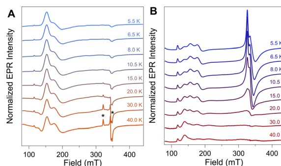
Fig. 3 CW EPR spectra ( \nu = 9.37 GHz, P_{\text{MW}} = 20 mW) of (A) NiFd-CN and (B) NiFd-CO at the indicated temperatures. Spectra were normalized to temperature using a standard Curie dependence [ I \propto T ]. * denotes small ( <5\% ) amount of contaminating S = 1/2 [\text{Fe}_4\text{S}_4]\text{-CN Fd} .
