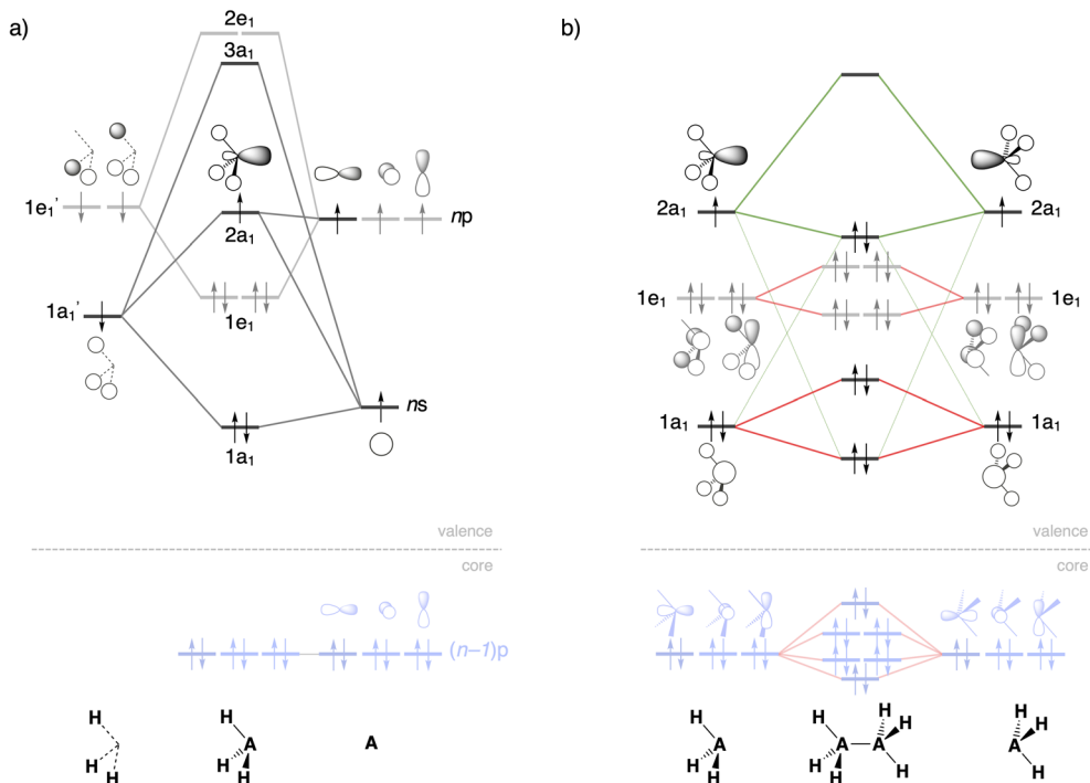
Fig. 3 Schematic molecular orbital diagrams of (a) pyramidal H 3 A + and (b) H 3 A-AH 3 (A = C, Si). Core Si 2p orbitals are highlighted in light blue, A-A electron-pair bond and donor-acceptor interactions in green, occupied-occupied orbital repulsion in red. MO numbering starts at the lowest-energy valence AO combination.
