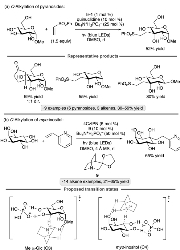
Scheme 51 Site-selective C -alkylations of pyranosides and myo-inositol, and proposed transition state structures for selective HAT. Ir-1 denotes [\text{Ir}(\text{d}(\text{CF}_3)_2\text{ppy})_2(\text{dtbbpy})]\text{PF}_6 ; 4CzIPN denotes 1,2,3,5-tetrakis(carbazol-9-yl)-4,6-dicyanobenzene.
