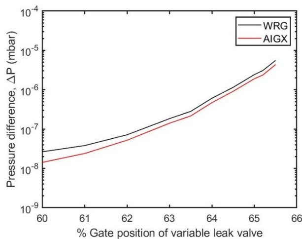
Figure 2. Pressure difference generated between the two sides of the diffusion channel as measured by the WRG (black) and AIGX (red) pressure gauges depending on the gate position of the leak valve. The gate position of the valve can be linked with the applied molar flux.
