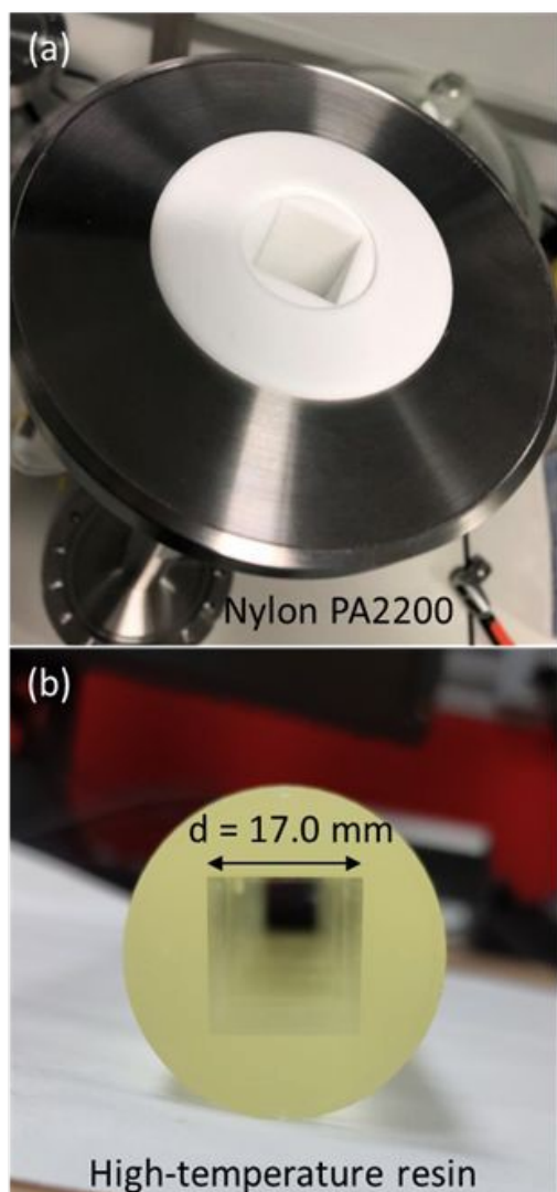
Figure 9. Photographs of two channels with a square cross section with edge length of 17 mm and channel length of 500 mm, made of: (a) PA2200 nylon using an SLS EOS Formiga P100 3D printer, and (b) high-temperature resin using an SLA Formlabs Form 3 3D printer.
