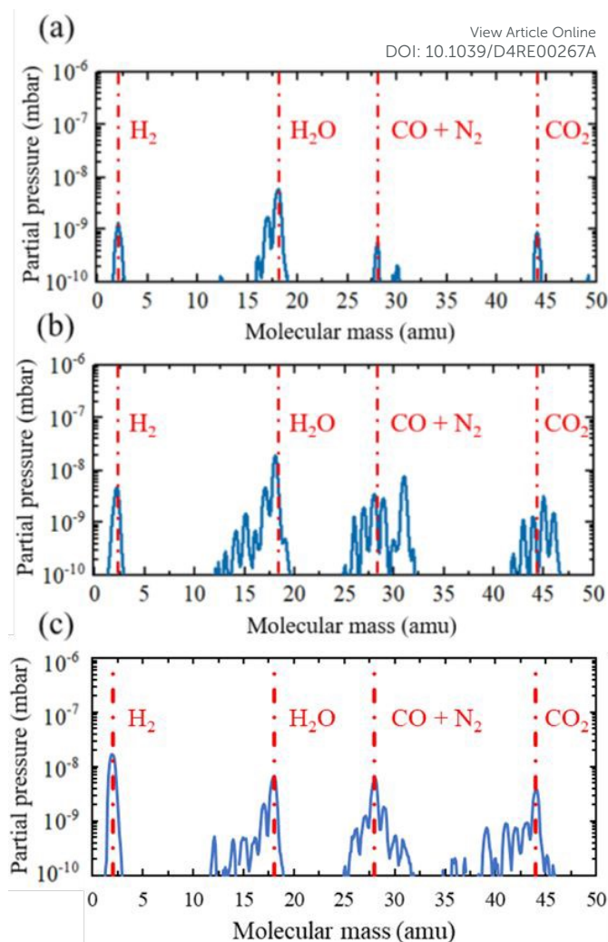
Figure 8. Mass spectral analysis of the gas species that are present in the UHVDS: (a) “empty” system; (b) a pre-treated PA2200 nylon segment of L = 50 mm fabricated by the SLS EOS Formiga P100 3D printer, and (c) a pre-treated high-temperature resin channel of L = 500 mm fabricated by the SLA Formlabs Form 3 3D printer inserted inside the diffusion channel. The analysis is conducted using the SRS RGA100 mass spectrometer.
