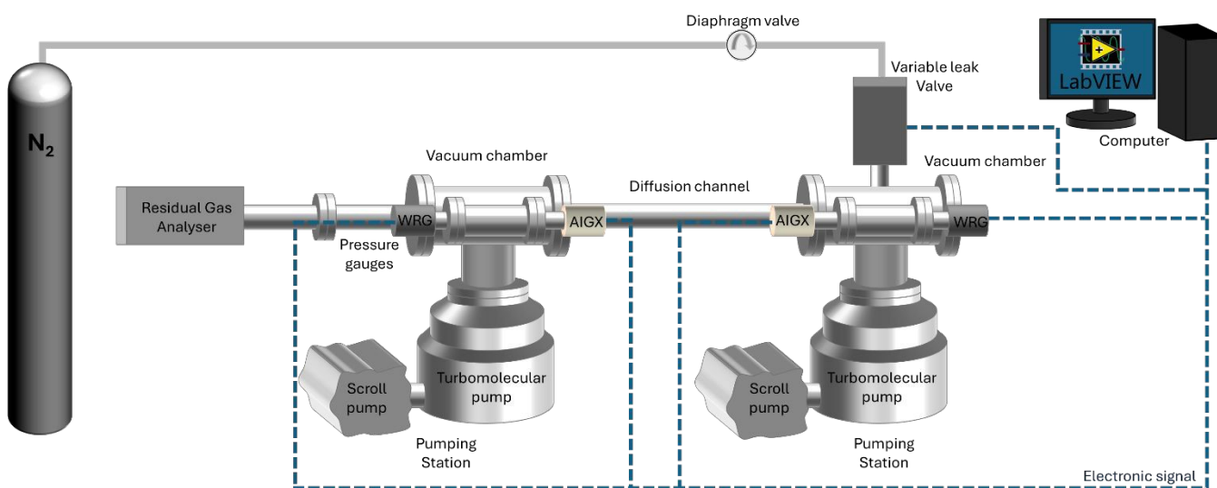
Figure 1. Schematic representation of the UHVDS and its components.
