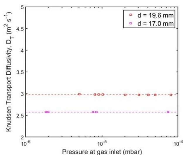
Figure 10. Knudsen transport diffusivity for the square channels with 19.6 mm (red squares) and 17.0 mm (pink squares) hydraulic diameter and 500 mm length for varying pressure at the gas inlet using the UHVDS.
