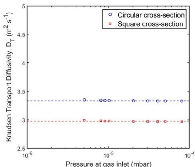
Figure 6. Knudsen transport diffusivity for the channels with circular (blue circles) and square (red squares) cross section for varying pressure gradient at the gas inlet using the UHVDS.
