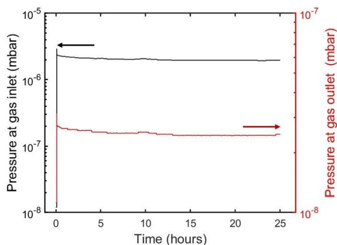
Figure 3. Pressures at the gas inlet and outlet of the pore channel, as measured by the hot cathode (AIGX) pressure gauge (note the different log scales for the inlet and outlet).
