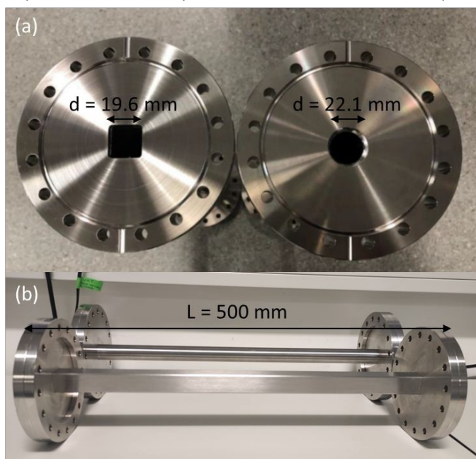
Figure 7. Photographs of two stainless-steel channels of: (a) varying pore shape with a square and a circular cross section of the same area, and (b) same pore length of L = 500 mm.
