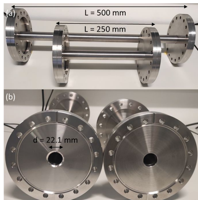
Figure 4. Photograph of stainless-steel channels with: (a) varying length of 250 mm and 500 mm, and (b) circular cross section with the same diameter of 22.1 mm.
