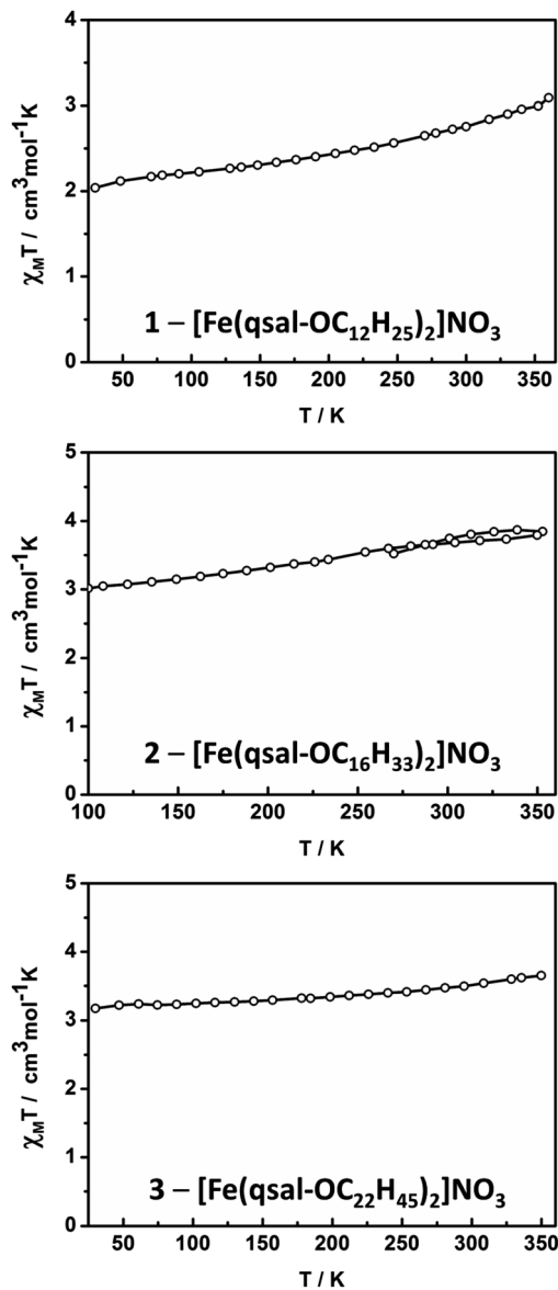
Fig. 5 \chi_M T vs. T plots for 1–3.
