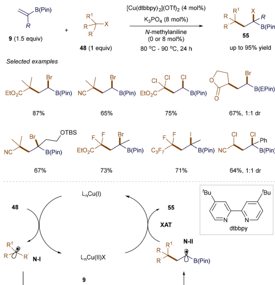
Scheme 20 ATRA reaction.
