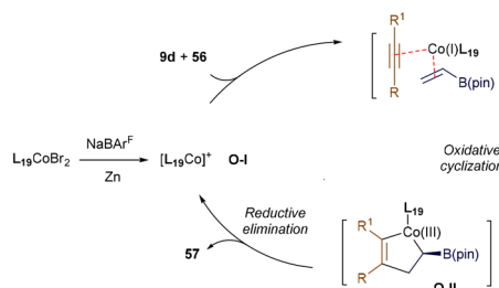
Scheme 21 Co(I)-catalyzed [2 + 2] cycloaddition.
