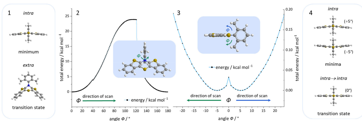
Fig. 3 Visualization of the relaxed geometry PES scans of N -inversion (2) and ring inversion (3) of N -aryls by the angle \phi of 3i (B3LYP/6-311G**, IEFPCM \text{CH}_2\text{Cl}_2 ). Most relevant minimum and transition state geometries of the relaxed geometry PES scan of N -inversion (1) and ring inversion (4) (B3LYP/6-311G**, IEFPCM \text{CH}_2\text{Cl}_2 ).
