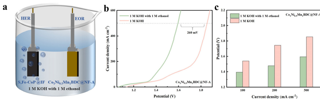
Fig. 7 (a) Schematic diagram of a two-electrode system. (b) Comparison of the polarization curves for \text{Co}_1\text{Ni}_{0.5}\text{Mn}_1\text{BDC}@NF-A during water splitting in 1 M KOH with and without 1 M ethanol and (c) the potentials at different current densities.
