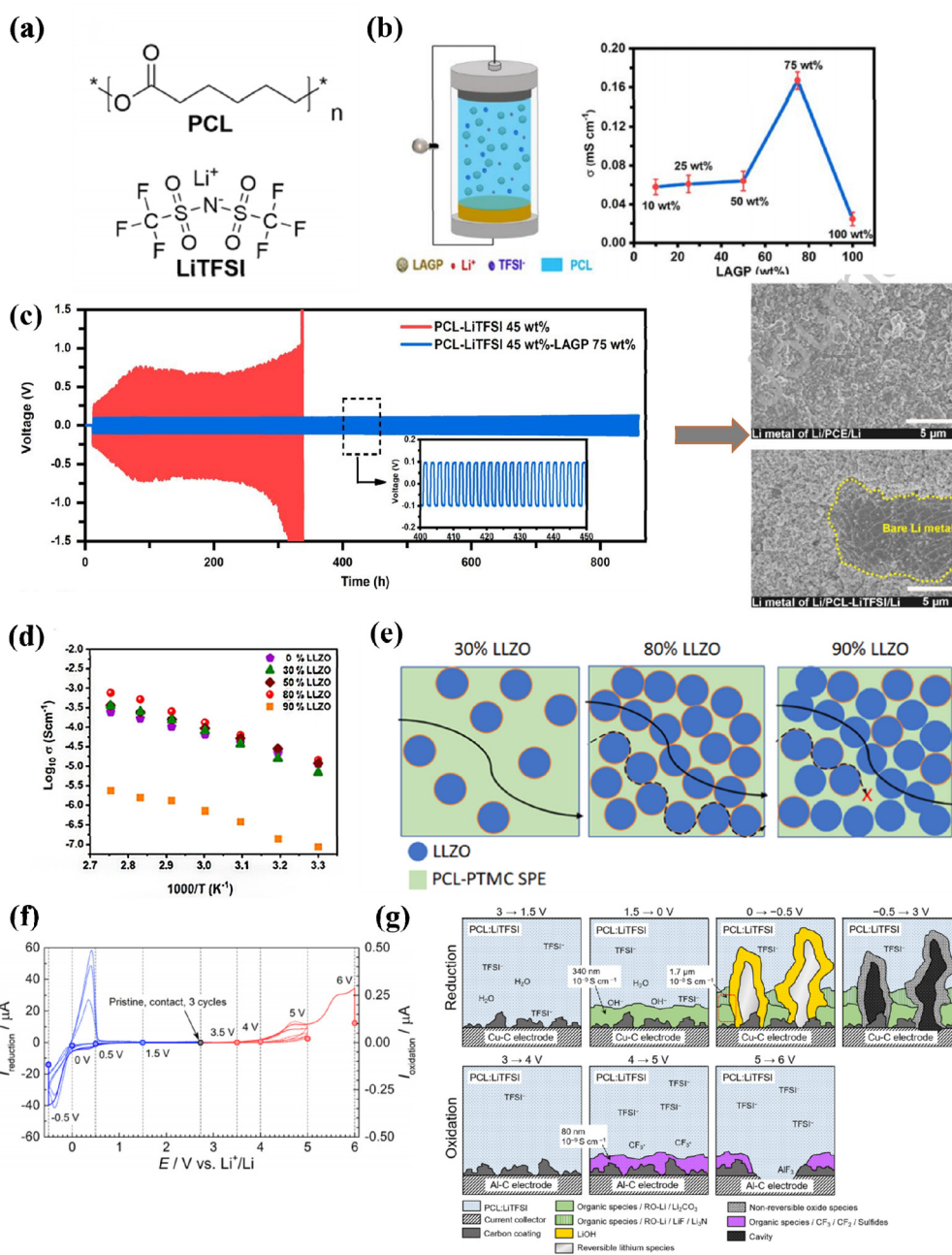
Fig. 8 (a) Structure of poly( \epsilon -caprolactone) ref. 127. Copyright 2015, Elsevier. (b) Ionic conductivity of the composite electrolyte, (c) Galvanostatic tests of Li/PCL-LiTFSI 45 wt%-LAGP 75 wt% Li and Li/PCL-LiTFSI 45 wt% Li cells at a constant current density of 0.1 \text{ mA cm}^{-2} (ref. 126). Copyright 2021, Elsevier. (d) Comparison of Arrhenius plots for the ionic conductivity of the polymer and composite electrolytes with different LLZO loadings, (e) schematic representation of the Li-ion transport in composite electrolytes at 30 wt% LLZO, 80 wt% LLZO, and 90 wt% LLZO loadings ref. 129. Copyright 2021, Elsevier. (f) Current profiles of Li/PCL: LiTFSI/Cu-C or Al-C cells taken apart for postmortem morphological and compositional analysis, current response during linear sweep to different cutoff potentials followed by a potential hold for 3 h (solid line) and during the first three cycles, (g) schematic of solid polymer electrolyte-electrode interface at different potentials. Interfacial layer thickness and ionic conductivity are based on calculations that assume that the interfacial layer covers 50% of the electrode area ref. 127. Copyright 2015, Elsevier.
