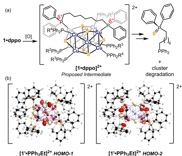
Fig. 7 (a) Proposed pathway for decomposition of [\text{Cu}_{12}\text{S}_6] via oxidative \text{P}=\text{S} bond formation. (b) Calculated HOMO-1 and HOMO-2 (DFT: BP86/def2-SVP) of [1'\text{-PPh}_2\text{Et}]^{2+} showing significant \text{S}_{3p} orbital character on nearby bridging sulfides.
