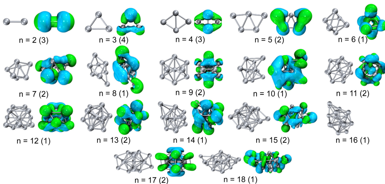
Fig. 4 Lowest energy structures and spin states of neutral (Al)_n clusters calculated with DFT using CAM-B3LYP. The numbers in parenthesis correspond to the spin state of the cluster. Charge carrier transition densities of the hole (blue) and electron (green) for the excited state accessed with the pump (3.1 eV) photon. As the charge carriers spread over larger distances, the presented isovalue also decreases (0.002 for clusters Al_2 – Al_4 , 0.001 for Al_5 – Al_9 , 0.0005 for Al_{10} – Al_{17} , and 0.0004 for Al_{18} ) for representation.
