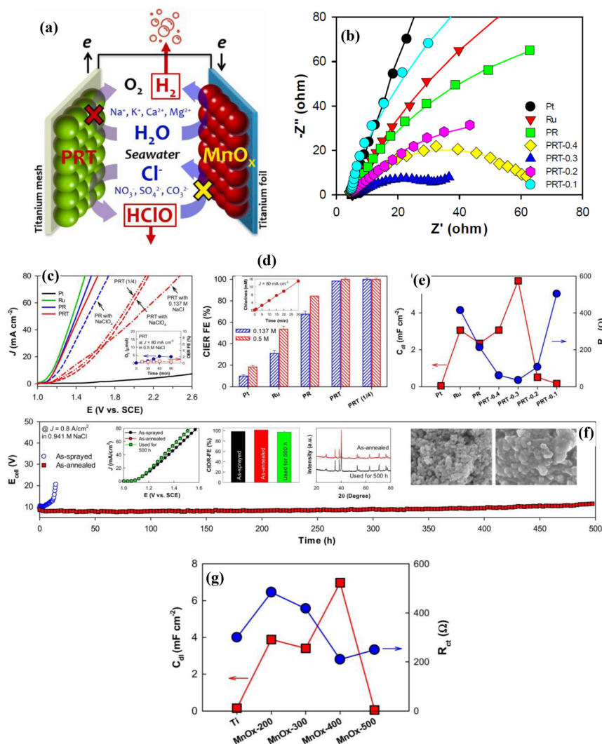
Fig. 7 (a) Schematic diagram illustrating seawater electrolysis using the MnO x cathode and PtRuTiO x (PRT) anode without using a membrane in a single compartment cell, where the CIOR selective anode and HER selective cathode could eliminate the CIOR, while pure H 2 gas could be formed, where the chlorine generated could be in the aqueous form. (b) Nyquist plot of Pt 0.06 Ru 0.24 Ti 0.7 O y in comparison with those of its counterparts for CIOR in simulated seawater electrolyte. (c) LSV curves for CIOR of PRT in comparison with those of its counterparts in 0.5 M NaCl (pH 6), 0.137 M NaCl and 0.5 M NaClO 4 (pH 6), where PRT (1/4) indicates a mass loading of 0.83 mg cm -2 , while the inset depicts the CIOR and faradaic efficiency (FE) of PRT at 80 mA cm -2 in 0.5 M NaCl. (d) FE of PRT in comparison with those of its counterparts for CIOR at 80 mA cm -2 , where the inset depicts the production of free chlorine over time at 80 mA cm -2 . (e) R ct and C dl values obtained from the Nyquist plot of Pt 0.06 Ru 0.24 Ti 0.7 O y in comparison with those of its counterparts in simulated seawater electrolyte. (f) Long-term stability test for CIOR of as-annealed PRT in comparison with that of as-sprayed PRT at 80 mA cm -2 in 0.941 M NaCl, where the inset depicts the LSV curves and FE for CIOER of the as-sprayed and as-annealed materials and PRT used for 500 h at 80 mA cm -2 in 0.5 M NaCl, while the inset further shows the XRD patterns of the as-annealed material and PRT used for 500 h, and the inset further depicts the SEM images of the as-annealed material (left) and PRT used for 500 h (right). (g) R ct and C dl values obtained from the Nyquist plot of MnO x -400 in comparison with those of its counterparts for the HER in simulated seawater electrolyte (reproduced with permission from ref. 25. Copyright 2022, Elsevier B.V.).
