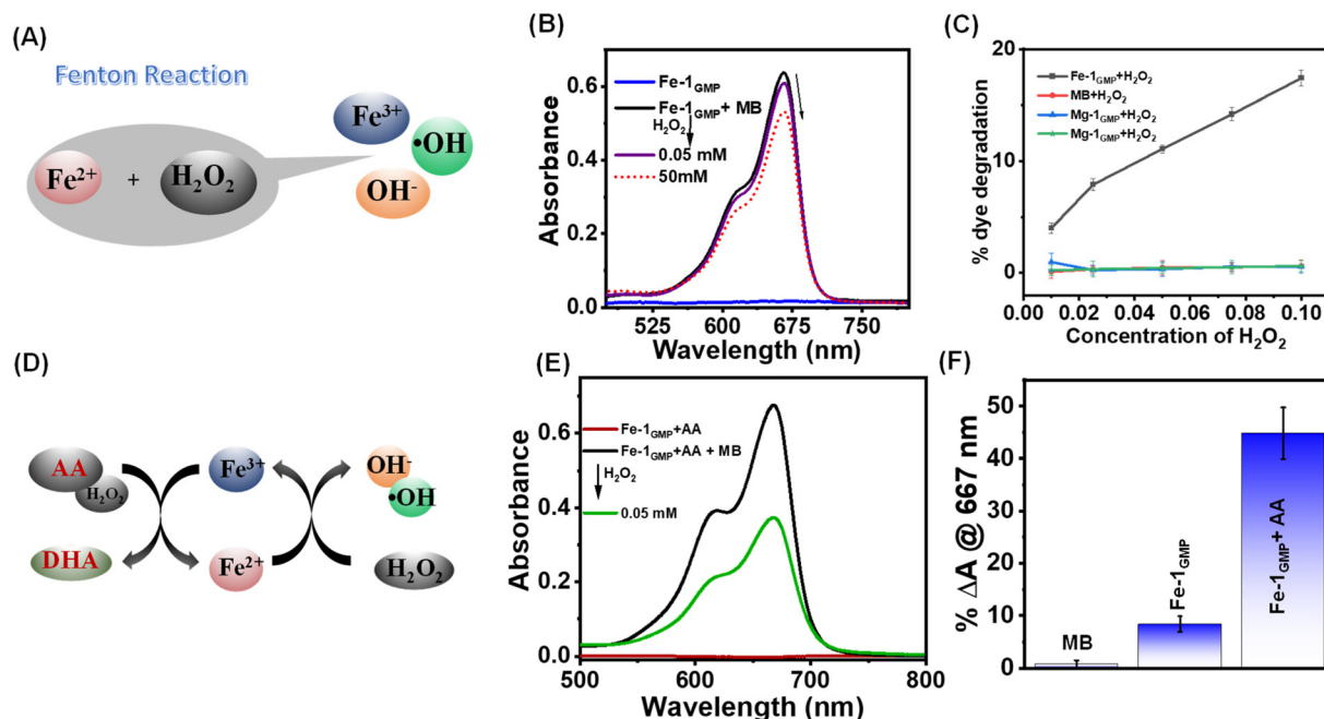
Fig. 4 (A) Schematic representation of the Fenton reaction illustrating the conversion of ferrous ions ( \mathbf{Fe^{2+}} ) and hydrogen peroxide ( \text{H}_2\text{O}_2 ) into ferric ions ( \mathbf{Fe^{3+}} ), hydroxyl radicals ( \cdot\text{OH} ), and hydroxide ions ( \text{OH}^- ). (B) UV-vis spectra depicting changes in the absorption of the \mathbf{MB} dye following successive additions of \text{H}_2\text{O}_2 solution to \mathbf{Fe-1_{GMP}} . (C) Comparison with respect to dye degradation in different hydrogels. (D) Schematic illustration of the role of ascorbic acid in increasing the production of reactive oxygen species (ROS). (E) UV-vis spectra showing enhanced degradation of \mathbf{MB} after the addition of AA to \mathbf{Fe-1_{GMP}} . (F) Comparison of the percentage dye degradation of \mathbf{Fe-1_{GMP}} and \mathbf{Fe-1_{GMP} + AA} by addition of 0.05 mM \text{H}_2\text{O}_2 .
